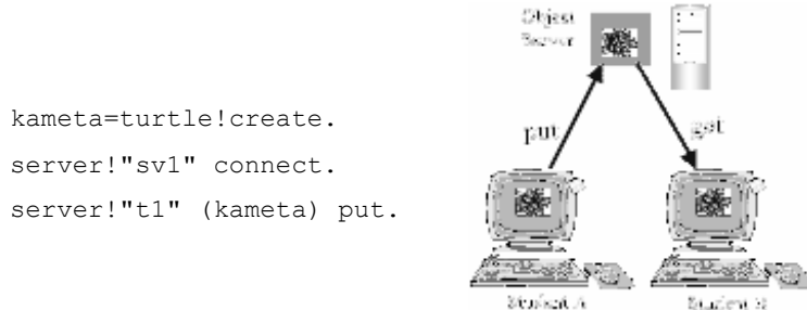
Figure 11. Registering, cloning objects
